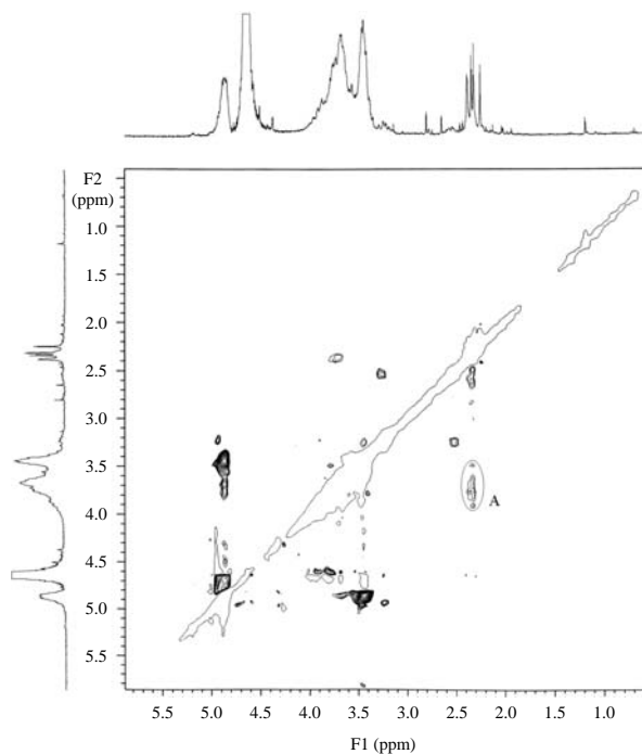
Figure 2. ROESY spectrum of 3 in D 2 O at 25°C ( [\mathbf{3}] = 1.0 \times 10^{-3} M). Peak A was assigned to the NOE correlations between -\text{SCH}_3 protons and the interior protons of the CD cavity.
