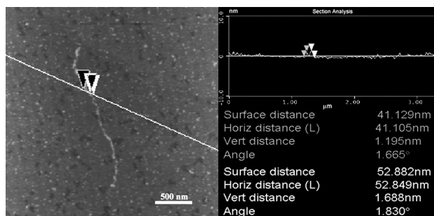
Figure 6. AFM image of the ternary supramolecular polymer of HBV 4+ @CB[8]/bisSC4A scale bar = 500 nm.
