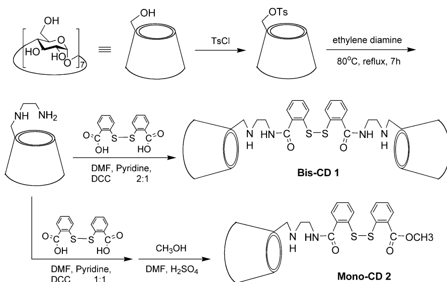
Scheme 1. Synthetic routes of host CDs.
