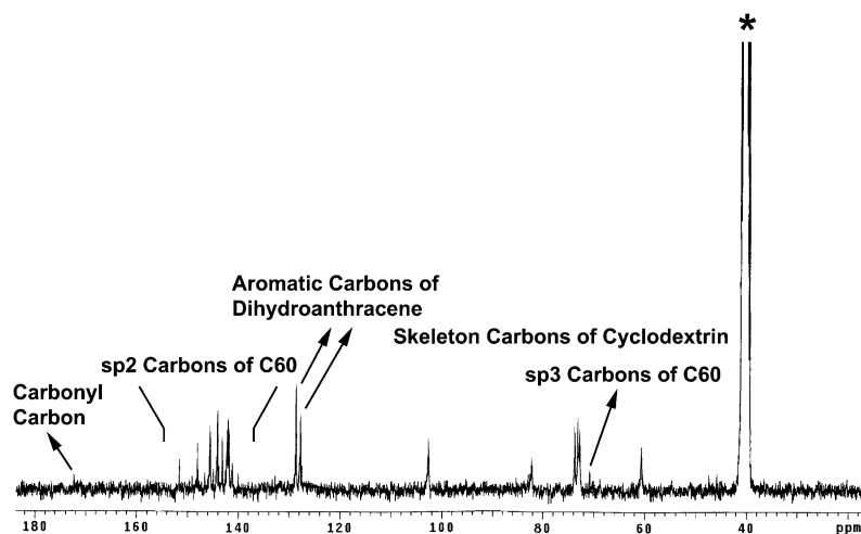
Figure 3. The ^{13}\text{C} NMR spectrum of 2 ( 2.1 \times 10^{-3} M) in \text{DMSO-}d_6 at 25^\circ\text{C} .
