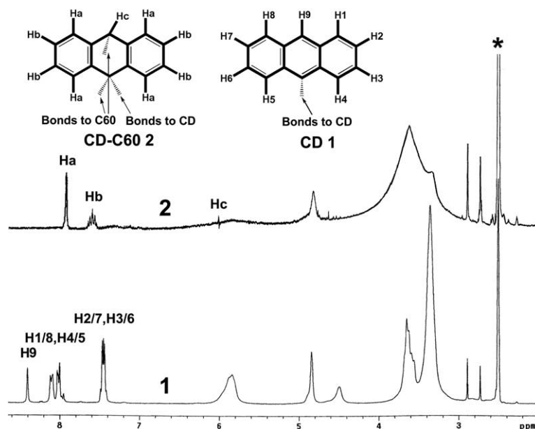
Figure 2. ^1\text{H} NMR spectra of 1 ( 4.2 \times 10^{-3} M) and 2 ( 4.4 \times 10^{-3} M) in \text{DMSO-}d_6 at 25^\circ\text{C} .
