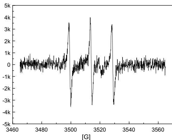
Figure 5. The EPR spectrum of a mixture of 2 ( 1.5 \times 10^{-4} M) with TEMP ( 9.2 \times 10^{-3} M) after the visible-light irradiation in an aqueous phosphate buffer solution (pH 7.4, containing 5% DMF) at 298 K.
