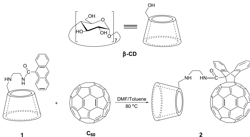
Scheme 1. Synthetic route of CD- C_{60} conjugate 2 .
