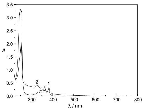
Figure 1. The UV-vis spectra of 1 ( 1.4 \times 10^{-5} M) and 2 ( 1.2 \times 10^{-5} M) in aqueous solution at 25 °C.
