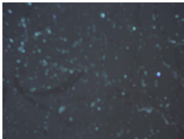
Figure 7. Fluorescence micrograph (magnification 400 \times ) of 2 /NaDC mixture ([NaDC] = 10 mM, [ 2 ] = 0.6 mM) in buffer solution (pH 9.18).
