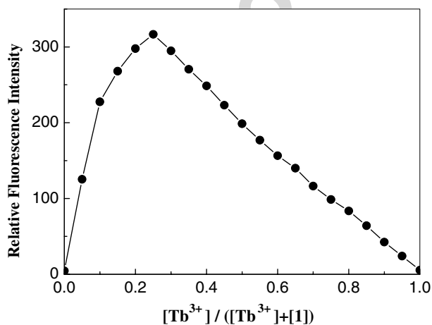
Figure 1. Job's plot of 1/ Tb^{3+} system in aqueous buffer solution at 25 °C and pH 9.18 ( [1] + [Tb^{3+}] = 1.0 \times 10^{-5} M) produced with data taken from fluorescence spectra ( \lambda_{ex} = 275 nm, \lambda_{em} = 492 nm).
