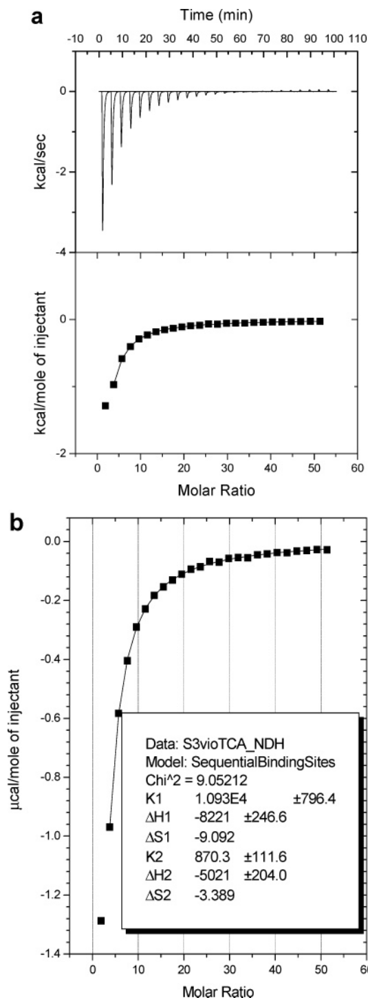
Figure 1. (a) Heat effects of complexation of benzyl viologen ( BV^{2+} ) with thiacalix[4]arenesulfonate for each injection during the titration microcalorimetric experiment. (b) "Net" heat effect obtained by subtracting the heat of dilution from the heat of reaction, which was analyzed by computer simulation using the two sequential two binding sites model.
