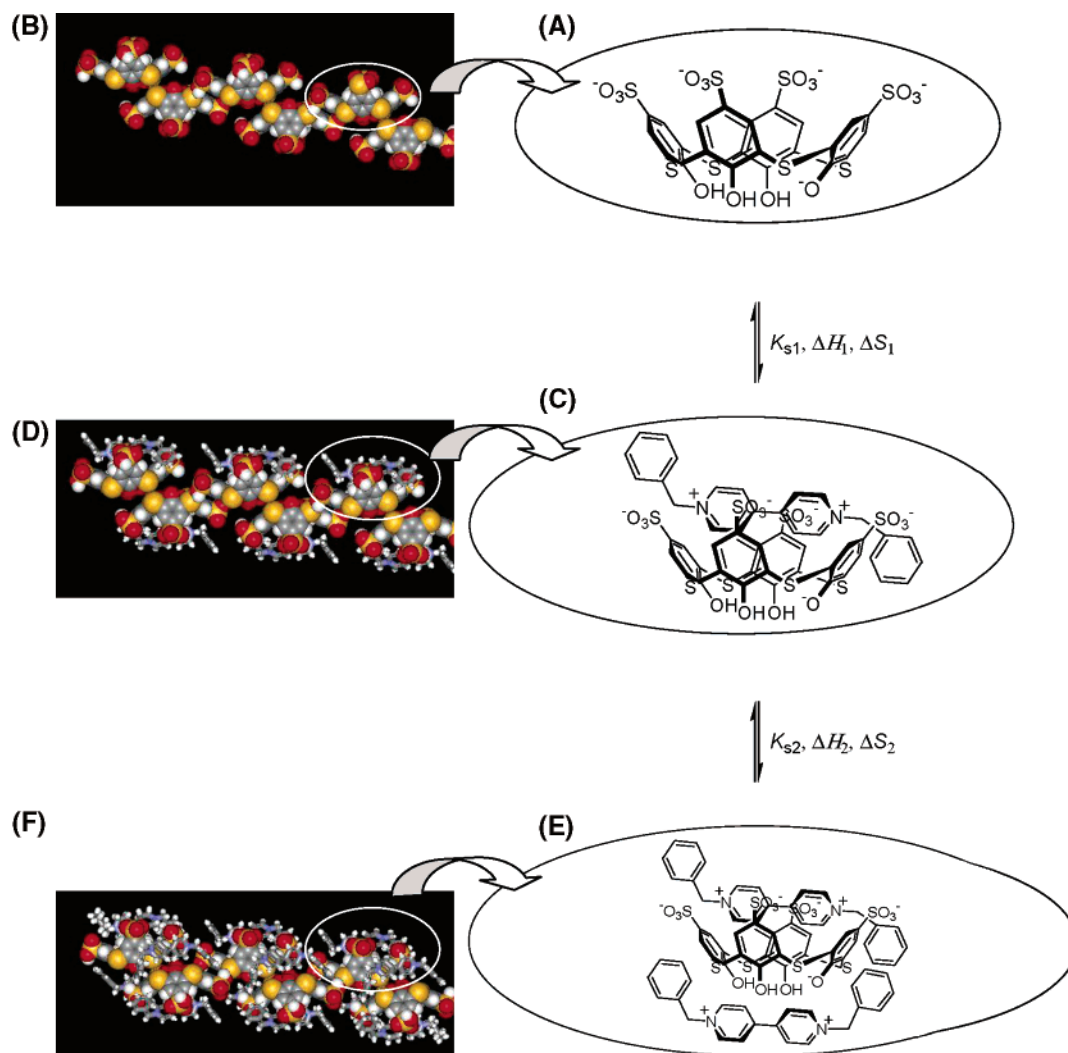
Figure 5. Schematic representation of the self-assembly of (A) p -sulfonatothiacalix[4]arene anions STCA into the layer structure (B) morphologies (hydrated sodium ions and water molecules were omitted for clarity). (C) In the presence of a guest, the first BV^{2+} molecule is included into the hydrophobic cavity of thiacalix[4]arenesulfonate. (D) BV^{2+} molecule located on the surfaces of the layer. (E) With the addition of BV^{2+} , the second binding site on the lower rim of the thiacalix[4]arenesulfonate. (F) BV^{2+} molecules intercalated into the organic layer in the second step binding process through van der Waals and electrostatic interactions. In the representation, p -sulfonatothiacalix[4]arene anions are shown in space-filled view and BV^{2+} molecules are in stick models. Elements are colored as follows: C, gray; H, white; N, blue; O, red; and S, yellow.
