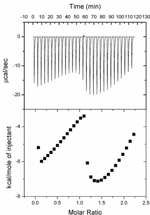
Figure 2. Two step binding of heat effects of complexation of benzyl viologen ( BV^{2+} ) ( 10.5 \text{ mmol} ) with thiacalix[4]arenesulfonate ( 1.06 \text{ mmol} ) for each injection during the titration microcalorimetric experiment.
