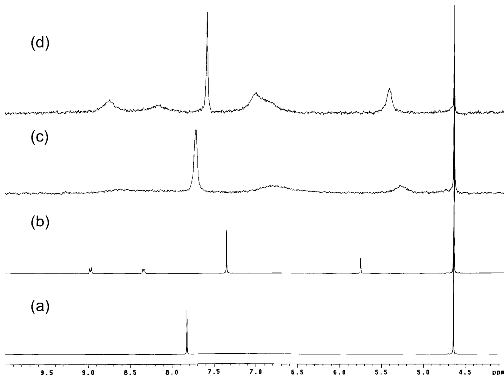
Figure 3. ^1\text{H} NMR spectra of (a) STCA, (b) \text{BV}^{2+} , (c) \text{STCA}:\text{BV}^{2+} = 1:1 (molar ratio), and (d) \text{STCA}:\text{BV}^{2+} = 1:2 (molar ratio).
