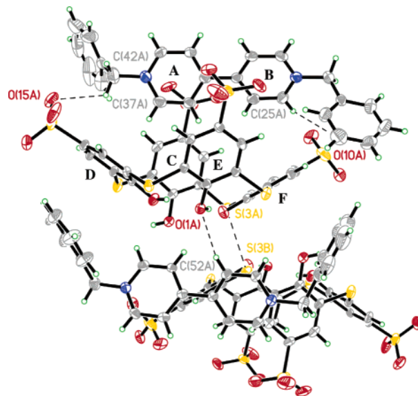
Figure 4. View of a section of the structure illustrating the arrangement of two \text{BV}^{2+} molecules. One is complexed by the hydrophobic cavity of the thiacalix[4]arenesulfonate. Rings A and B are sandwiched and \pi-\pi stacked by rings C and E of the host (the centroid distances and dihedral between the rings A–C and the rings B–E are 4.947 Å, 18.8°, 5.126 Å, and 18.4°) and are almost perpendicular to rings D and F of the host. \text{C}_{37} belonging to guest forms \text{C}-\text{H}\cdots\pi interactions with ring D (the distance and angle of \text{C}-\text{H}\cdots\pi are 2.827 Å and 165.8°). The cavity of calixarene from the ideal C_{4v} symmetry cone configuration to one of distorted C_{2v} symmetry. The S···S (trans) approaches are 8.0 and 13.4 Å. The other \text{BV}^{2+} molecule is seen to be intercalated into another layer of calixarene.
