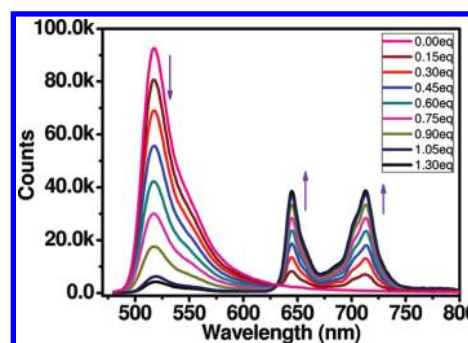
FIGURE 6. Fluorescence spectral changes of 1 ( 1 \times 10^{-6} M) upon addition of 2 in pH 7.2 phosphate buffer solution at 25 °C, \lambda_{\text{ex}} = 470 nm.
