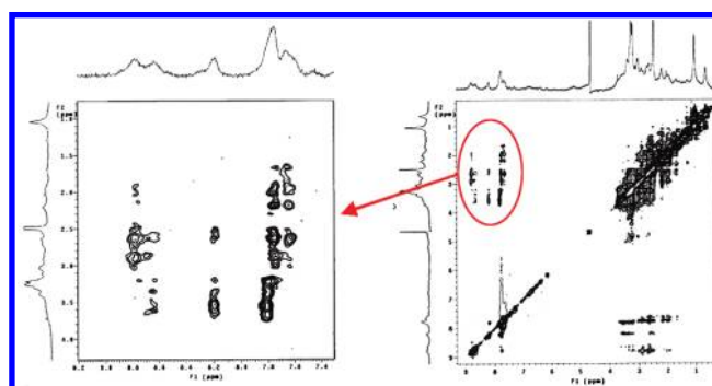
FIGURE 3. 2D NOESY spectra of 1 · 2 in 10% DMSO- d 6 -D 2 O at 25 °C with a mixing time of 220 ms.
