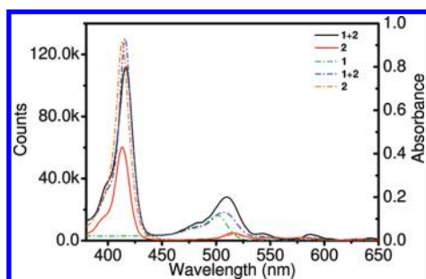
FIGURE 7. Excitation spectra of 1·2 and 2 (solid line) by monitoring the emission wavelength at 713 nm and absorption spectra of 1 , 2 , and 1·2 (dashed line) in pH 7.2 phosphate buffer solution at 25 °C; the concentration of 2 was 1 \times 10^{-6} M in excitation spectra and 5 \times 10^{-6} M in absorption spectra, respectively.
