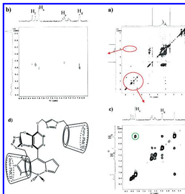
FIGURE 2. 2D NOESY spectra of 1 in 10% DMSO- d 6 -D 2 O at 25 °C with a mixing time of 220 ms. Panels b and c are enlarged areas of panel a. (d) Deduced structure of 1 .
