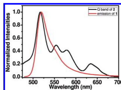
FIGURE 5. Normalized spectra of Q-band absorption of 2 and emission of 1 in pH 7.2 phosphate buffer solution at 25 °C.
