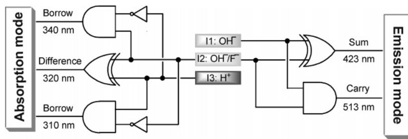
Figure 7. The corresponding electronic symbols of molecular half-adder and half-subtractor.
