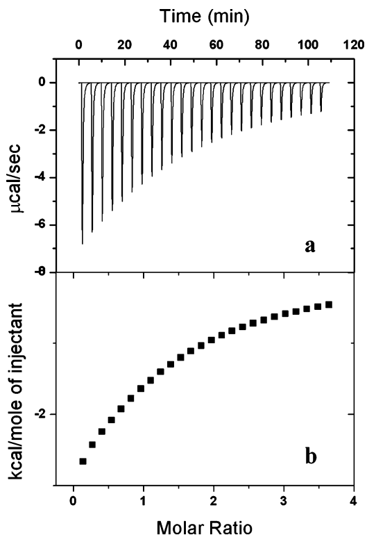
Figure 1. Microcalorimetric titration of C5AS with 2-DPD in phosphate buffer solution (pH = 2.0) at 298.15 K. (a) Raw data for sequential 25 injections (10 μL per injection) of C5AS solution (10.0 mM) injecting into 2-DPD solution (0.53 mM). (b) Apparent reaction heat obtained from the integration of calorimetric traces.
