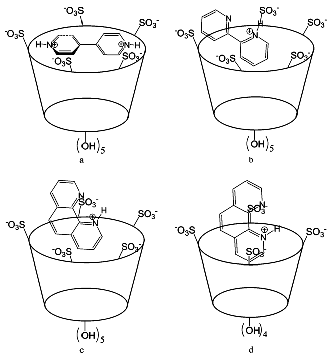
Figure 4. The deduced binding modes of guests with C5AS/C4AS hosts according to 2D NMR spectra.
