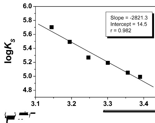
Figure 6. Plot of \log K_S vs 1/T in fluorimetric titration of amino-terminated PPG with host compound 2 at 20, 25, 30, 35, 40, and 45 °C.
