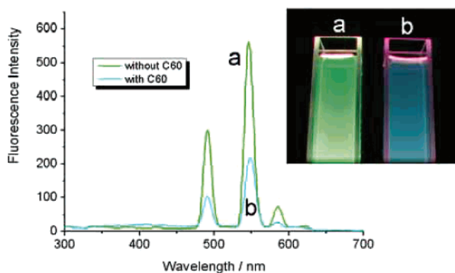
Figure 4. Luminescence spectra of polyad 2 and assembly 3 ( 1 \times 10^{-6} calculated as Tb^{3+} ) in a pH 7.2 Tris-HCl buffer solution; excitation wavelength: 275 nm, slit width 5 nm. (inset) Visible emission observed from (a) polyad 2 and (b) assembly 3 .
