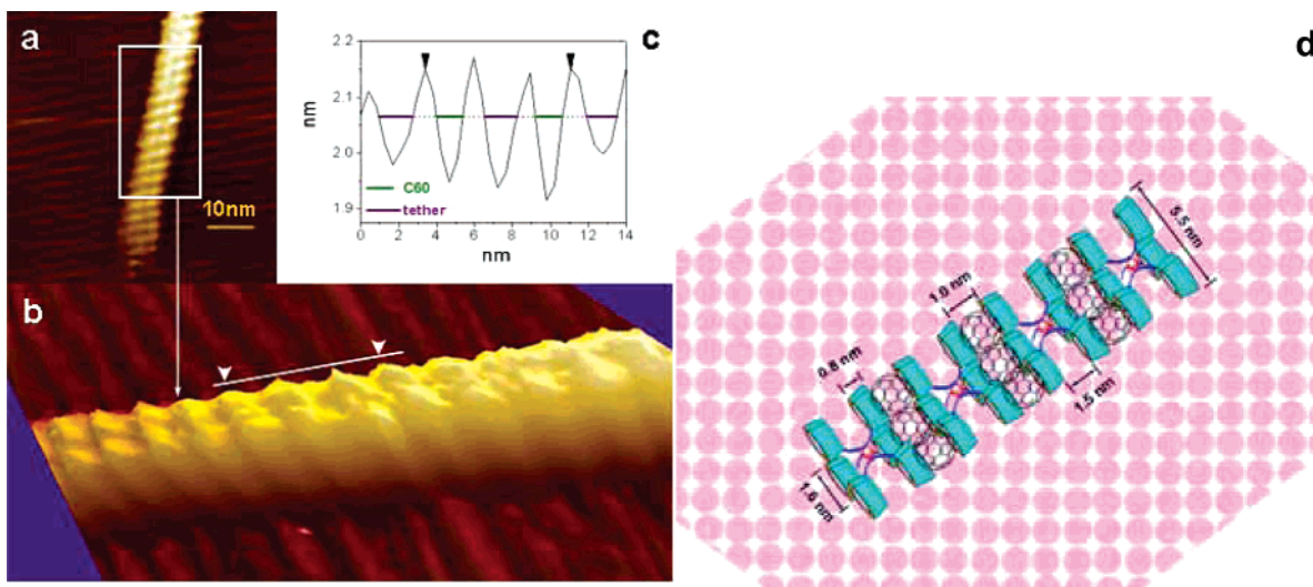
Figure 2. (a,b) STM images of assembly 3 on a HOPG surface (tunneling current 1.0 nA). (c) Line profile of image shown in (b). (d) Schematic structure of 3 .
