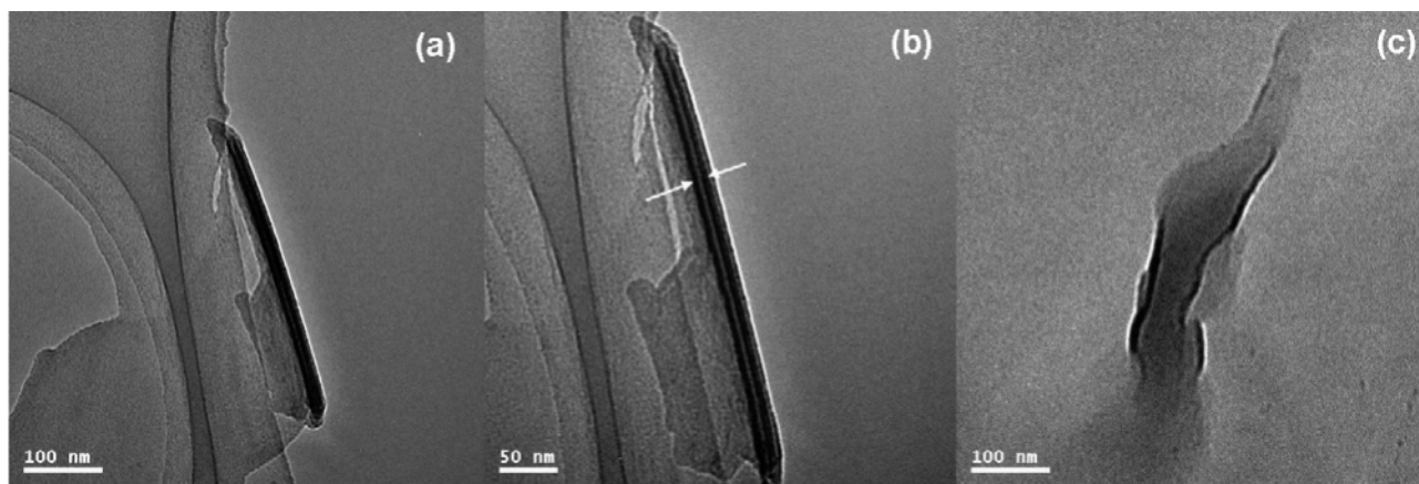
Figure 3. (a) TEM and (b) HR-TEM images of 3 ( 1 \times 10^{-4} M). (c) TEM images of 3 ( 5 \times 10^{-6} M).
