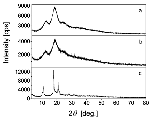
Figure 1. XRD patterns of (a) bis( \beta -CD) 1, (b) polyad 2, and (c) assembly 3.
