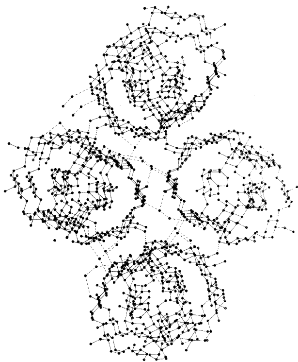
Figure 3. View down the columnar axis of 1 .
