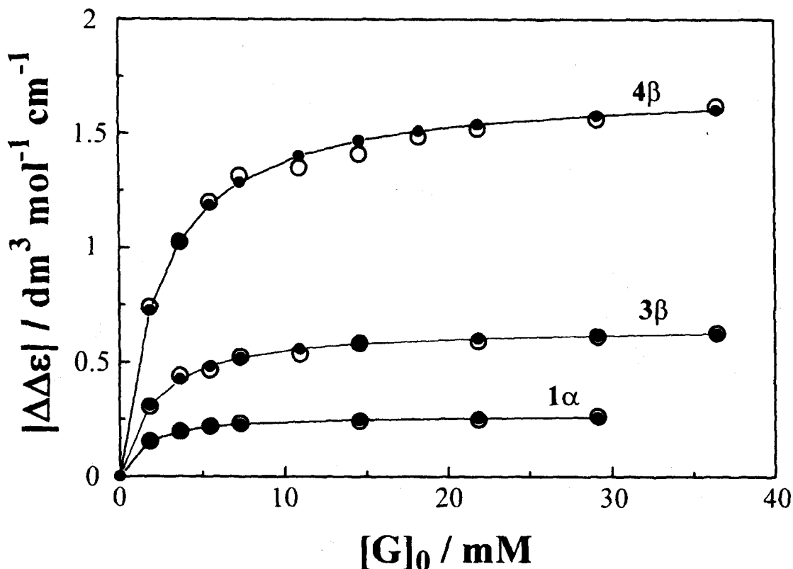
FIGURE 4 Curve-fitting analyses for complexations of cyclopentanol with 1\alpha , 3\beta , and 4\beta open circles represent experimental values, while dots denote calculated values
