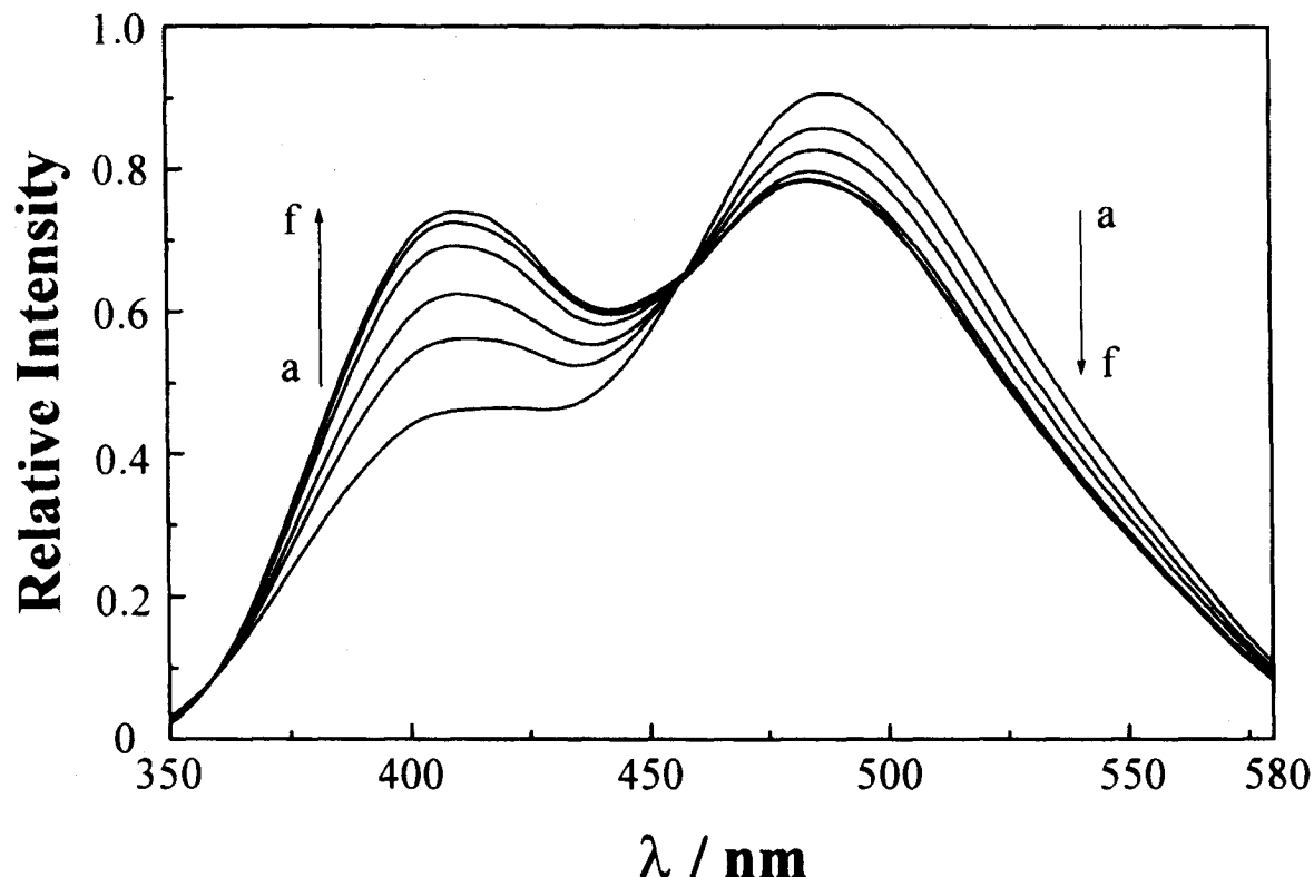
FIGURE 5 Fluorescence spectra of mono[6- O -(8-quinolyl)]- \beta -cyclodextrin ( 5\beta ) ( 10\ \mu\text{M} ) in phosphate buffer solution (pH 7.20) in the presence of various concentrations of 1-adamantanol: (a) 0, (b) 10, (c) 20, (d) 50, (e) 100, (f) 150\ \mu\text{M} ; excitation wavelength was 300 nm
