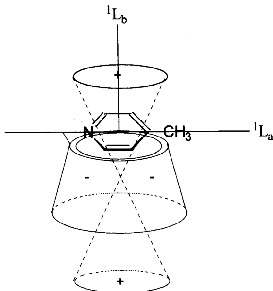
FIGURE 2 Kajtar's sector rule applied to transition moments of ^1L_a and ^1L_b bands of the p -picolinio moiety in 2\beta
