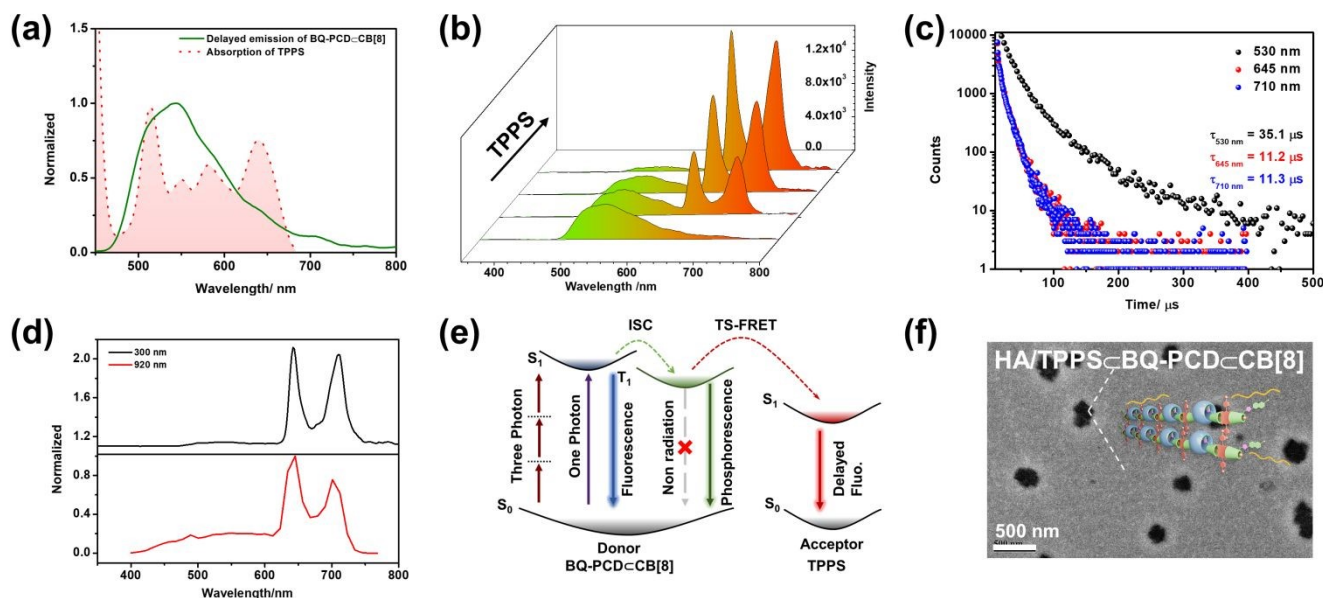
Fig. 3 (a) Normalized phosphorescence emission spectra of BQ-PCD=CB[8], and normalized absorption spectra of TPPS, (b) phosphorescence emission spectra of BQ-PCD=CB[8] in presence of variant concentrations of TPPS (delay time = 0.05 ms, [BQ-PCD] = 10 \mu M, [CB[8]] = 5 \mu M, [TPPS] = 0–6 \mu M, \lambda_{\text{ex}} = 300 nm), (c) time-resolved photoluminescence decay spectra of TPPS=BQ-PCD=CB[8] at 530 nm, 645 nm, 710 nm, (d) diagram of the possible mechanism for RTP energy transfer process (ISC = intersystem crossing, TS-FRET = triplet-to-singlet Förster resonance energy transfer), (e) emission spectra of TPPS=BQ-PCD=CB[8] excited at 300 (black curve) and 920 nm (red curve) ([BQ-PCD] = 10 \mu M, [CB[8]] = 5 \mu M, [TPPS] = 5 \mu M), (f) TEM images of HA/TPPS=BQ-PCD=CB[8].
