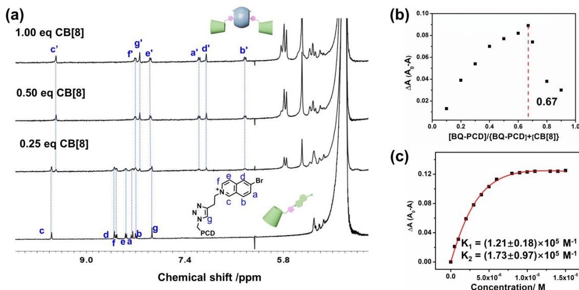
Fig. 1 (a) Partial 1 H NMR (400 MHz, D 2 O, 298 K) spectra of BQ-PCD and CB[8] ([BQ-PCD] = 1 mM, [CB[8]] = 0–1 mM), (b) Job plot showing 2:1 stoichiometry between BQ-PCD and CB[8] ([BQ-PCD] + [CB[8]] = 10 μM), (c) nonlinear curve fitting of absorption intensity change at 243 nm of BQ-PCD versus variant concentrations of CB[8] ([BQ-PCD] = 10 μM, [CB[8]] = 0–15 μM).
