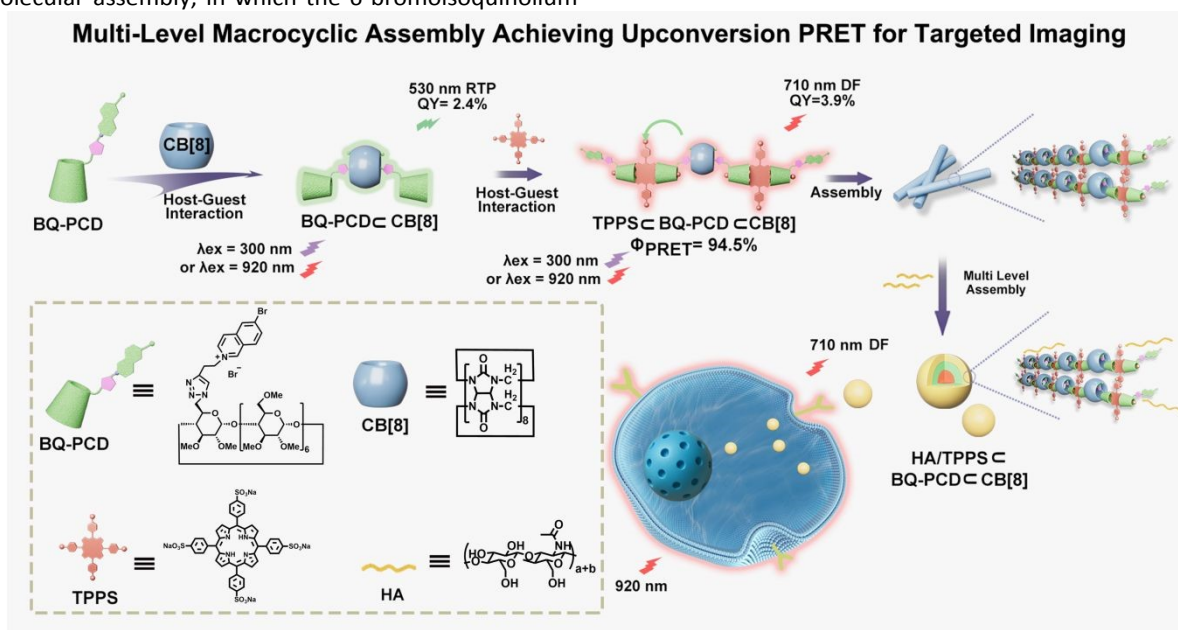
Scheme 1. Schematic illustration of multi-level macrocyclic assembly achieving organic upconversion PRET for targeting delayed fluorescence cell imaging.
