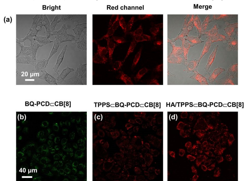
Fig. 4 (a) One-photon CLSM images of HeLa cells incubated with HA/TPPS \subset BQ-PCD \subset CB[8] ([BQ-PCD] = 10 \mu M, [CB[8]] = 5 \mu M, [TPPS] = 5 \mu M, [HA] = 20 \mu g/mL), three-photon CLSM images of HeLa cells incubated with (b) BQ-PCD \subset CB[8] (emission was collected at 500–580 nm, [BQ-PCD] = 10 \mu M, [CB[8]] = 5 \mu M), (c) TPPS \subset BQ-PCD \subset CB[8] (emission was collected at 620–740 nm, [BQ-PCD] = 10 \mu M, [CB[8]] = 5 \mu M, [TPPS] = 5 \mu M), (d) HA/TPPS \subset BQ-PCD \subset CB[8] (emission was collected at 620–740 nm, [BQ-PCD] = 10 \mu M, [CB[8]] = 5 \mu M, [TPPS] = 5 \mu M, [HA] = 20 \mu g/mL).
