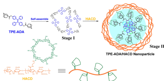
Scheme 1. Construction Process of TPE-ADA/HACD Nanoparticle
