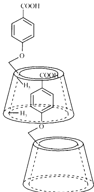
Fig. 5. The dimeric structure of 1 in aqueous solution.
