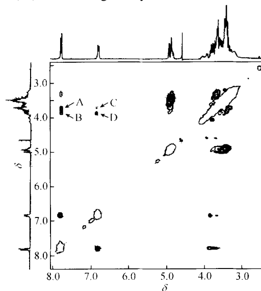
Fig. 4. 1 H ROESY spectrum (300 MHz) of 1 ([ 1 ] = 1.0 \times 10^{-3} mol/L) in D 2 O at 298 K with a mixing time of 300 ms.
