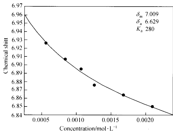
Fig. 6. Plot from ^1\text{H} NMR data of 1 as a function of total concentration to determine the aggregation equilibrium constant. The closed circles are the experimental data points, and the line is the theoretical curve based on the calculated values as equation d_{\text{obsd}} = d_m + f_d(d_m - d_a) =
