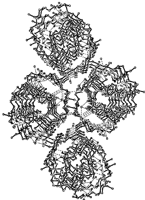
Fig. 3. The three-dimensional helical columnar structure.
