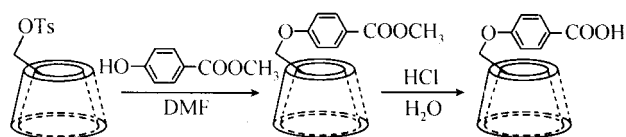
Fig. 1. The synthetic route of compound 1.
