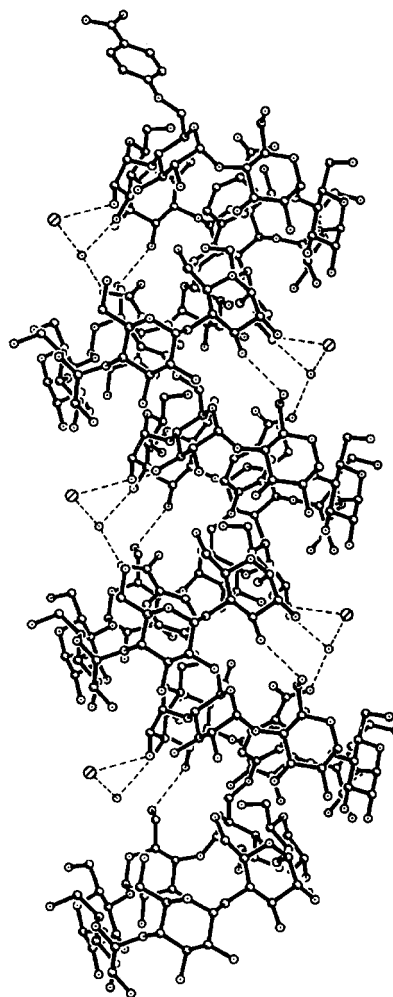
Fig. 2. Stereodrawing of the stacking structure of 1 .
