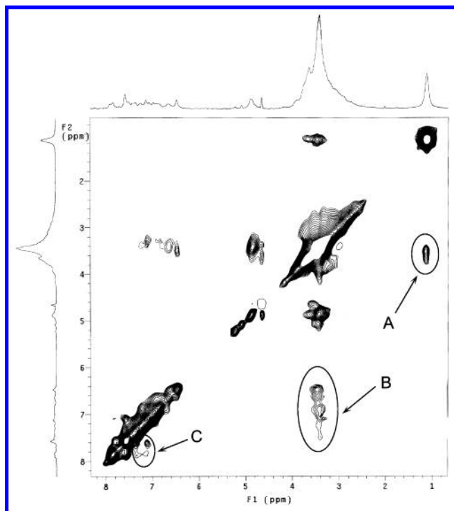
FIGURE 5. 1 H-NOESY spectrum (300 MHz) of a mixture of 4 with RhB ( [\mathbf{4}] = [\text{RhB}] = 5.0 \times 10^{-3} M) in D 2 O at 298 K with a mixing time of 600 ms.
