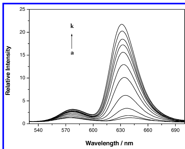
FIGURE 6. Fluorescence spectral changes of RhB (5.0 mM) upon addition of 4 (the concentration of host 4 : 0–6.7 mM from a to k).
