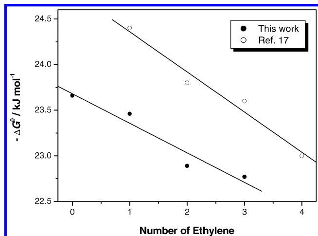
FIGURE 8. Plot of Gibbs free energy changes ( -\Delta G^\circ ) versus the ethylene number in the tether for the inclusion complexation of dimeric \beta -cyclodextrins 2–5 (●) and oligo(ethylenediamino)-bridged bis( \beta -cyclodextrin)s (○) with TNS.
