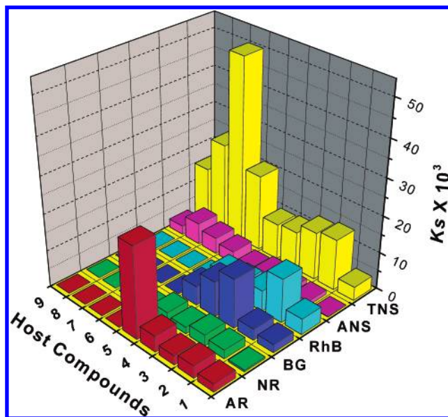
FIGURE 7. Complex stability constants ( K_S ) for the inclusion complexation of hosts 1–9 with guest molecules in aqueous solution.
