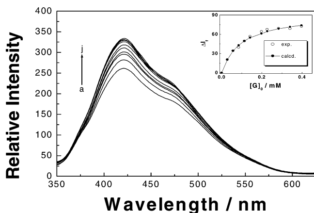
FIGURE 5. Fluorescence spectral changes of 1 ( 8.8 \times 10^{-6} M) upon addition of cholates in phosphate buffer solution (pH 7.20) at 25 °C. The concentrations of cholates are (0-4.0) \times 10^{-4} M, corresponding to traces a–j.
