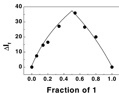
FIGURE 6. Job plot for the complexation of 1 with deoxycholate in phosphate buffer solution (pH 7.20) at 25 °C ( [1] + [\text{deoxycholate}] = 1.0 \times 10^{-5} M).
