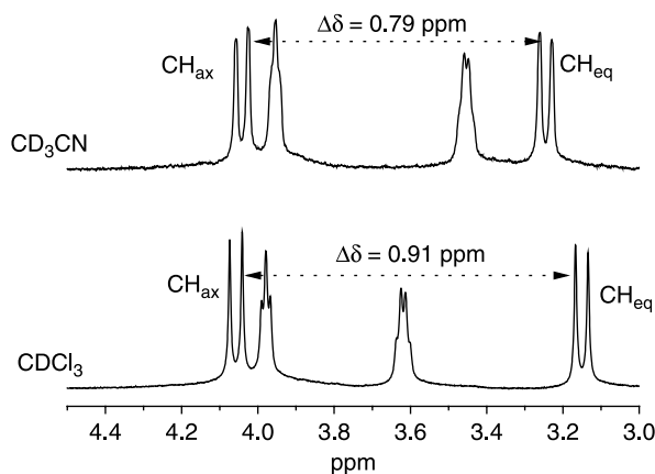
Figure 3. Partial ^1\text{H} NMR (400 MHz) of 3 (10 mM) in \text{CDCl}_3 and \text{CD}_3\text{CN} at room temperature.
