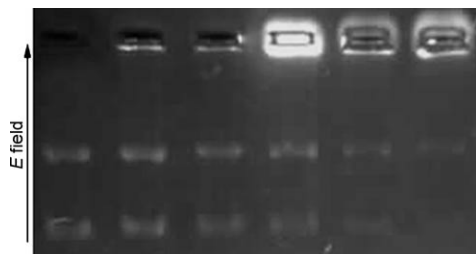
Figure 5. Agarose gel electrophoretogram of pUC19 plasmid DNA ( [DNA]=12.5 \text{ ng } \mu\text{L}^{-1} ) condensed with the supramolecular hybrid ( 1 ). From left to right: Lane 1, DNA only; lane 2–6, DNA + supramolecular hybrid ( [\text{hybrid}] = 150, 250, 500, 1000, \text{ and } 1250 \text{ ng } \mu\text{L}^{-1} , i.e., [\beta\text{-CD-RC}] = 0.03, 0.05, 0.10, 0.20, \text{ and } 0.25 \text{ mM} ). All samples are incubated at 25^\circ\text{C} in the dark for 1 h, 1 mM EDTA/10 mM Tris buffer, pH 8.0.
