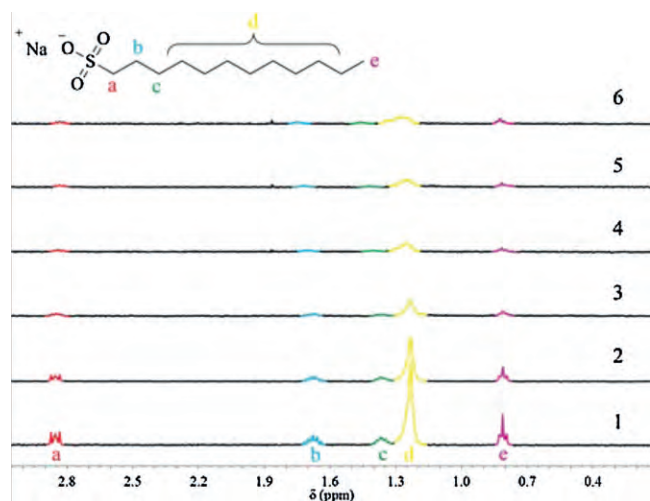
Fig. 2. Partial ^1\text{H} NMR spectra of SDS (1.0 mmol/L) with the increasing concentration of 3 in \text{D}_2\text{O} at 25 °C. From 1 to 6, [\mathbf{3}] = 0, 1.4 \times 10^{-5}, 1.0 \times 10^{-4}, 1.4 \times 10^{-4}, 2.0 \times 10^{-4}, and 3.3 \times 10^{-4} mol/L, respectively.
