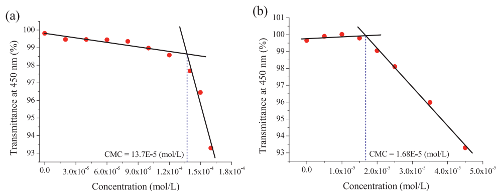
Fig. 1. Dependence of the optical transmittance of (a) SDS and (b) AOT at 450 nm in the presence of 0.04 mmol/L 3 at 25 °C.
