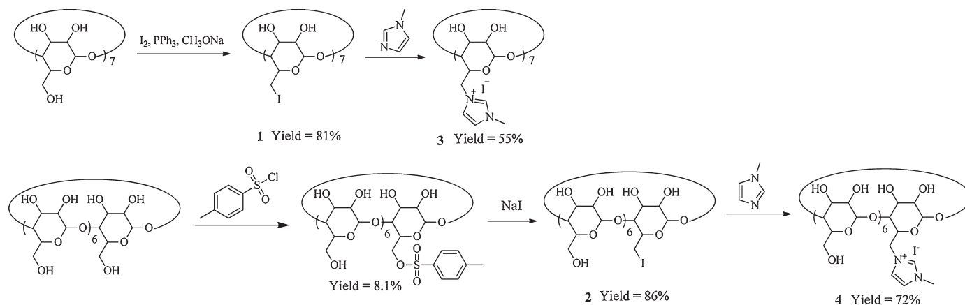
Scheme 1. Synthesis route of hosts 3 and 4 .
