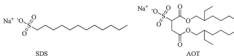
Scheme 2. Structures of guests SDS and AOT.
