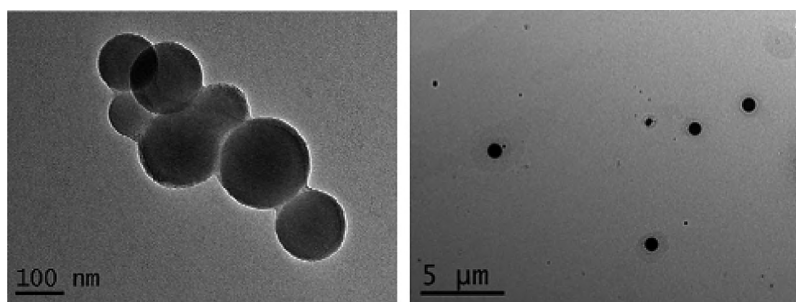
Fig. 5. TEM images of 3 /SDS (left) and 3 /AOT (right).
