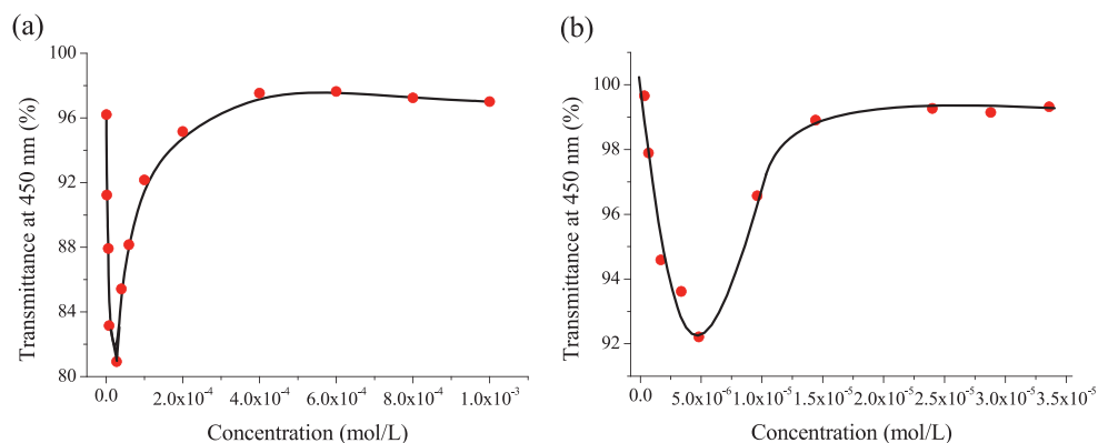
Fig. 3. Dependence of the optical transmittance (a) SDS (0.20 mmol/L) and (b) AOT (0.03 mmol/L) at 450 nm with increasing the concentration of 3 at 25 °C.
