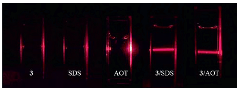
Fig. 4. Tyndall effect of 3 , SDS, AOT, 3 /SDS complex, and 3 /AOT in water at 25 °C, [ 3 ] = 1.4 \times 10^{-4} mol/L, [SDS] = [AOT] = 1.0 \times 10^{-3} mol/L.
