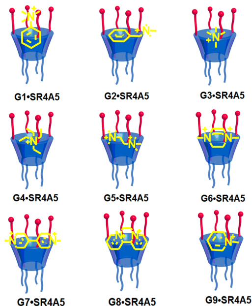
Figure 3. Possible binding modes of SR4A5 with guests G1–G9.
